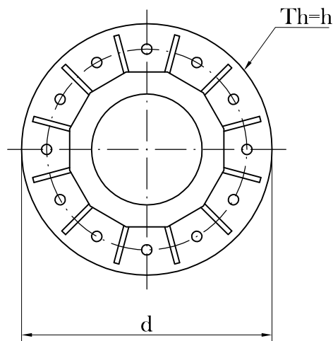
Base plate
